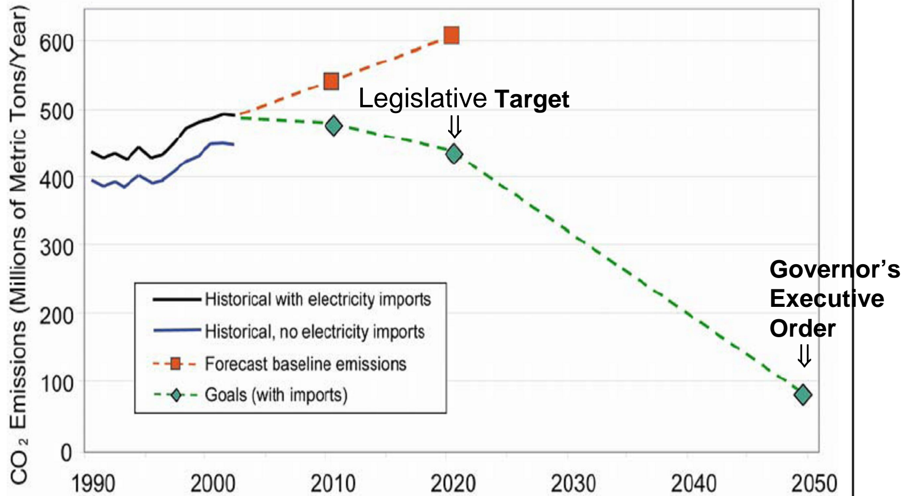
Figure 3. Historical and forecast greenhouse gas emissions, and California's goals. Source: Bemis and Allen (2005).
